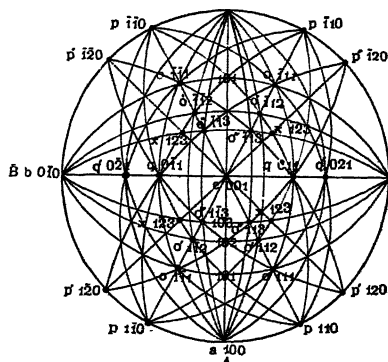
FIG. 54.—Stereographic Projection of Topaz.
